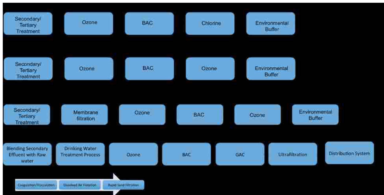
Figure 2 – Examples of potable reuse treatment trains throughout the world
